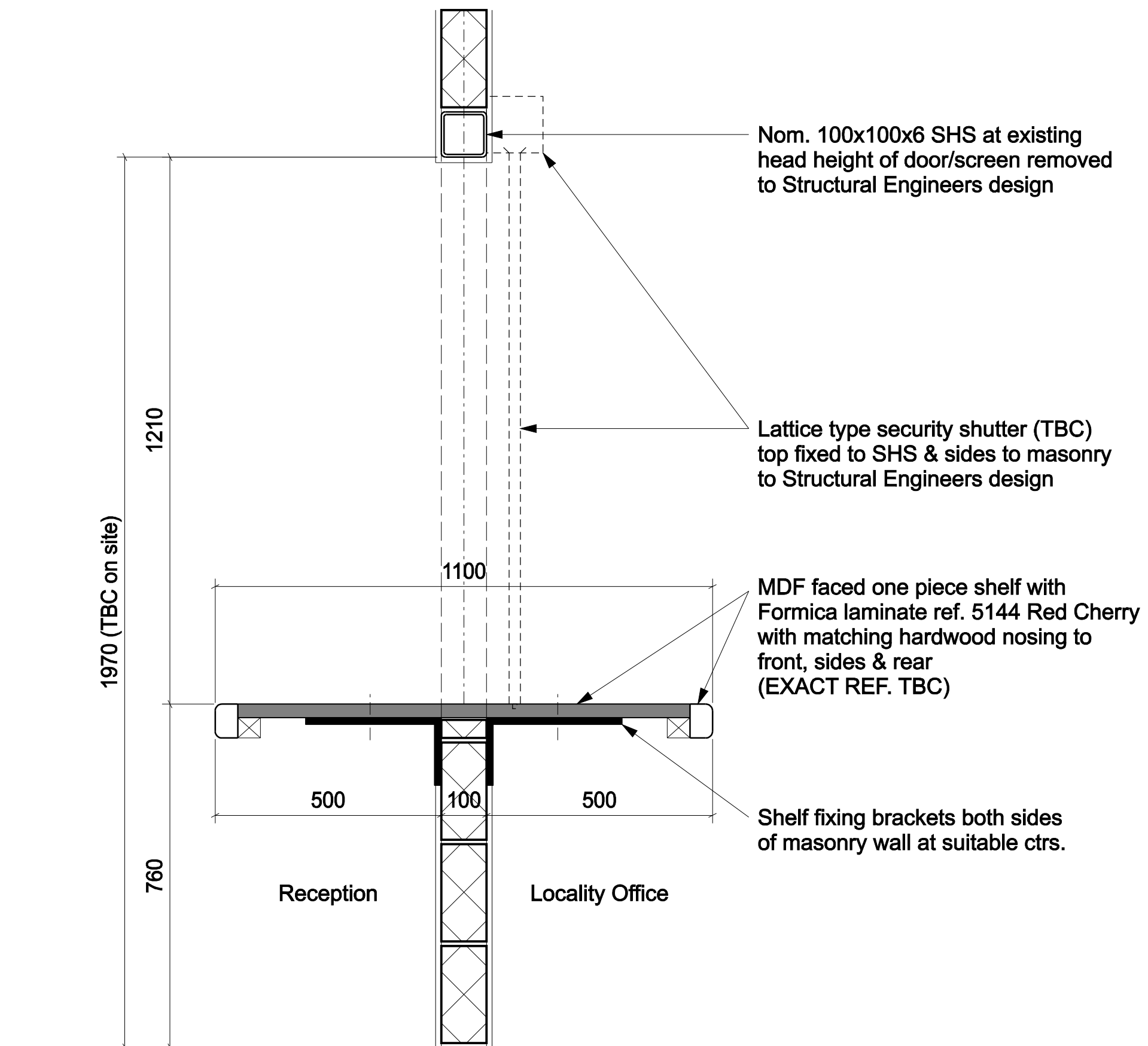
TYPICAL SECTION scale 1:10
