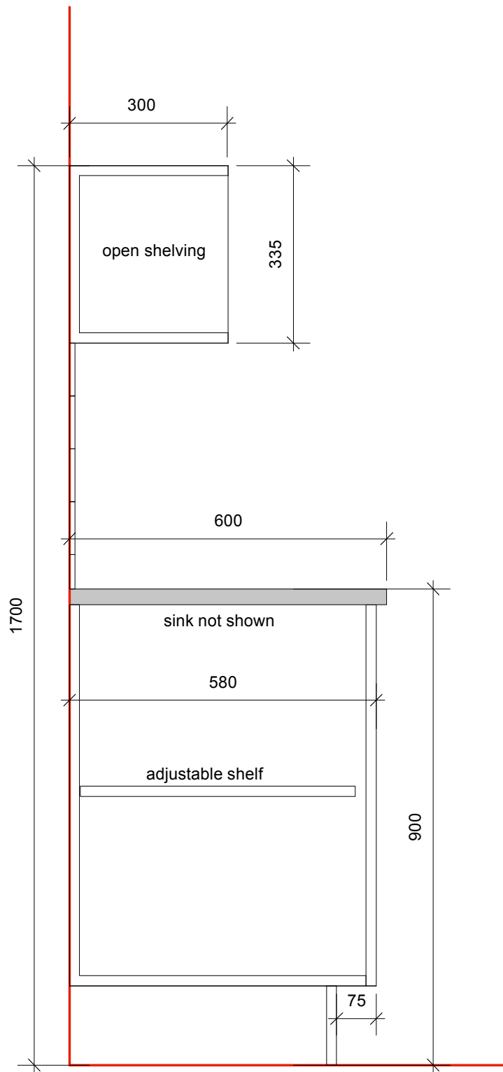
SECTION THROUGH HIGH LEVEL BASE UNIT
