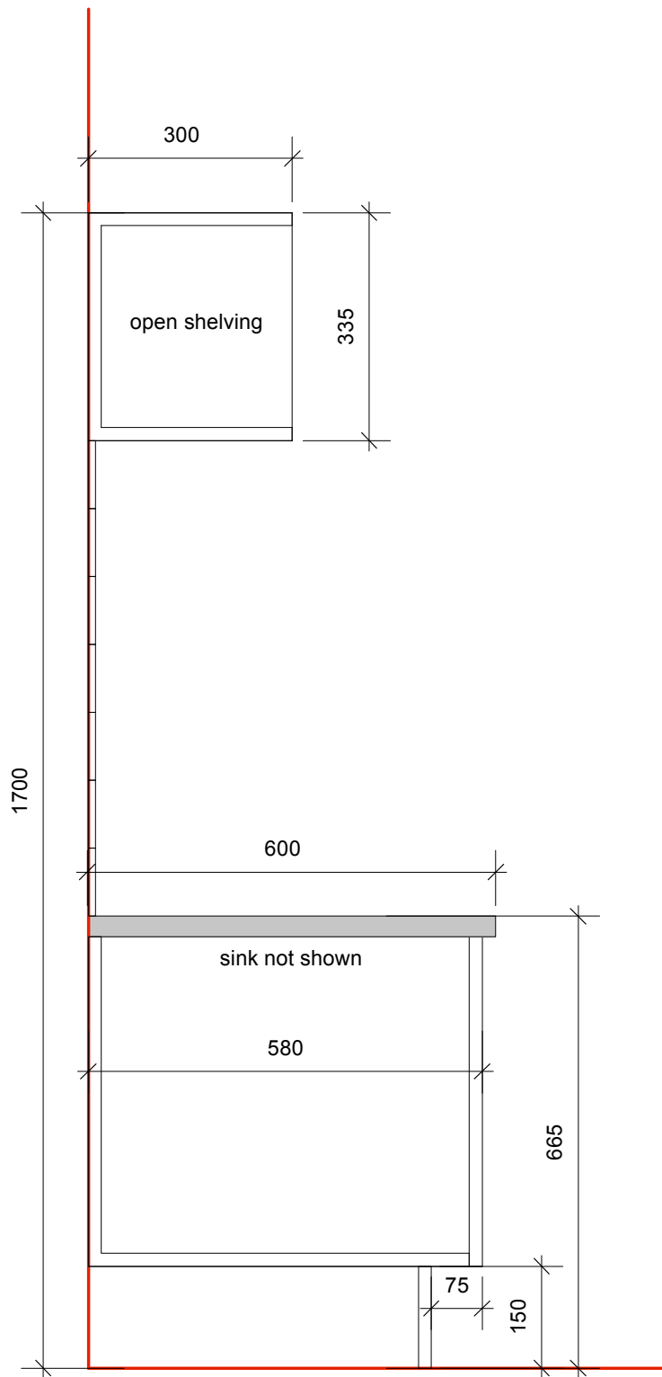
SECTION THROUGH LOW LEVEL BASE UNIT
