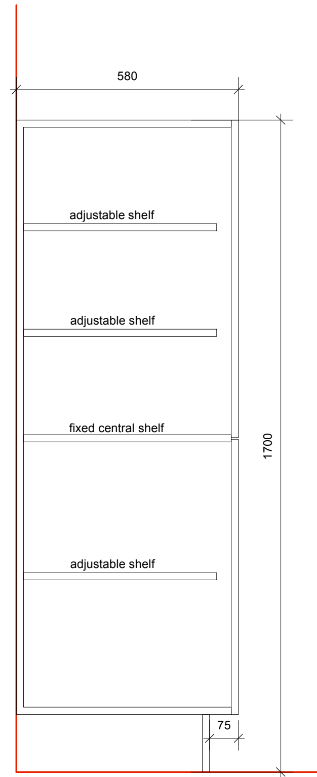
SECTION THROUGH TALL UNIT
