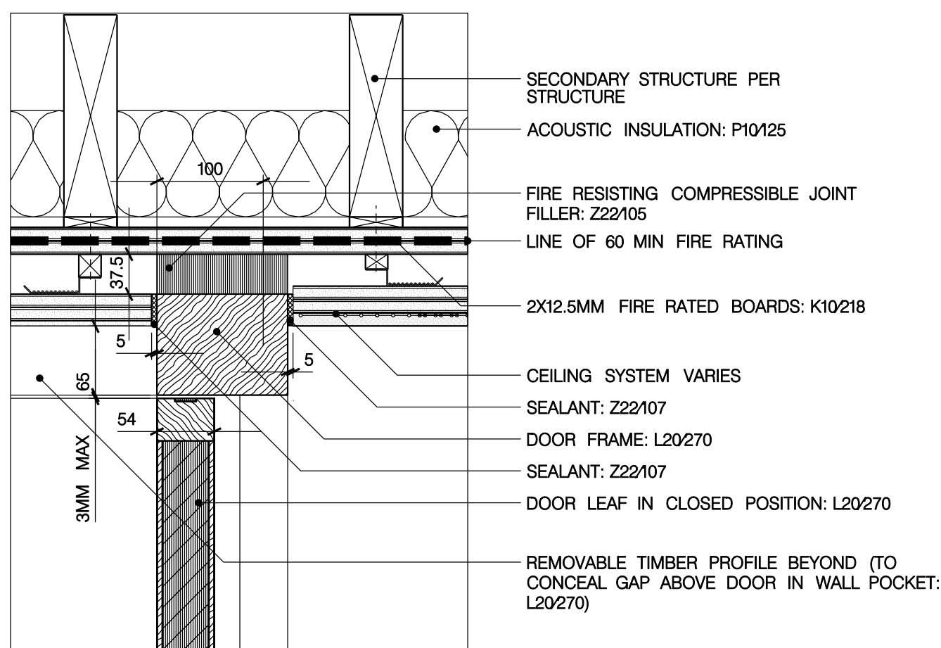
SECTION DETAIL HEAD DETAIL OF D-206-1, D-306-1
