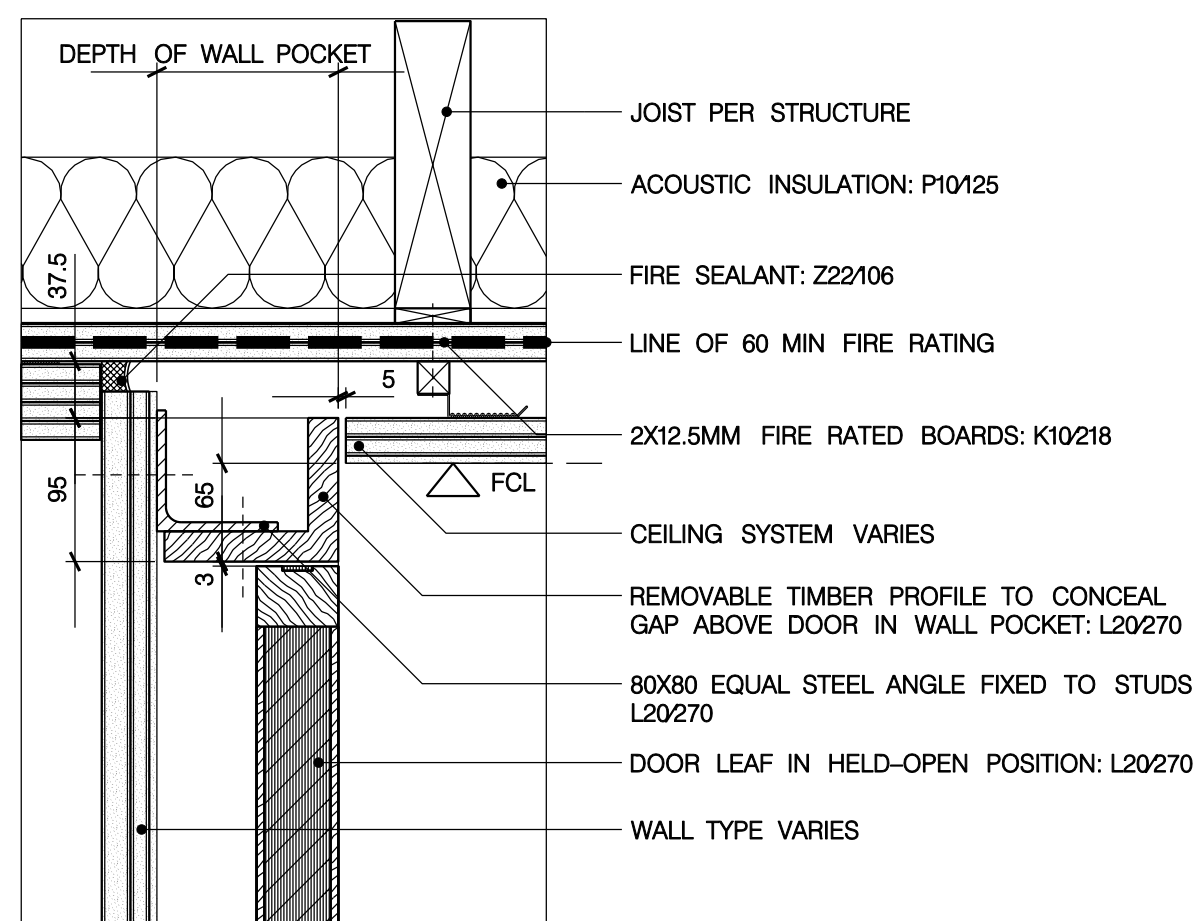
SECTION DETAIL HEAD DETAIL AT WALL POCKET OF D-206-1, D-201-1, D-203-2, D-306-1, D-301-1, D-303-1
