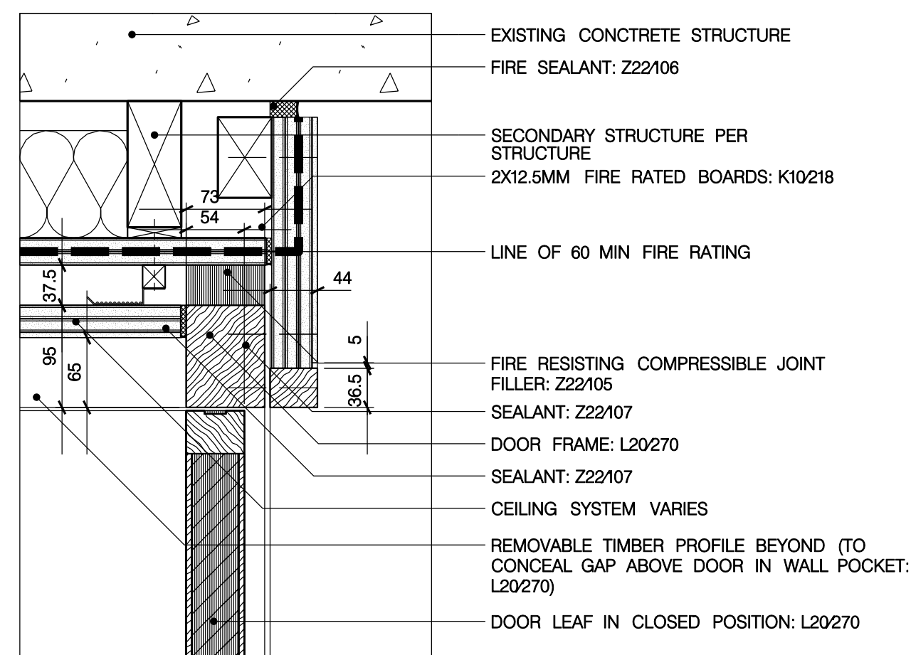
SECTION DETAIL HEAD DETAIL OF D-201-1, D-301-1
