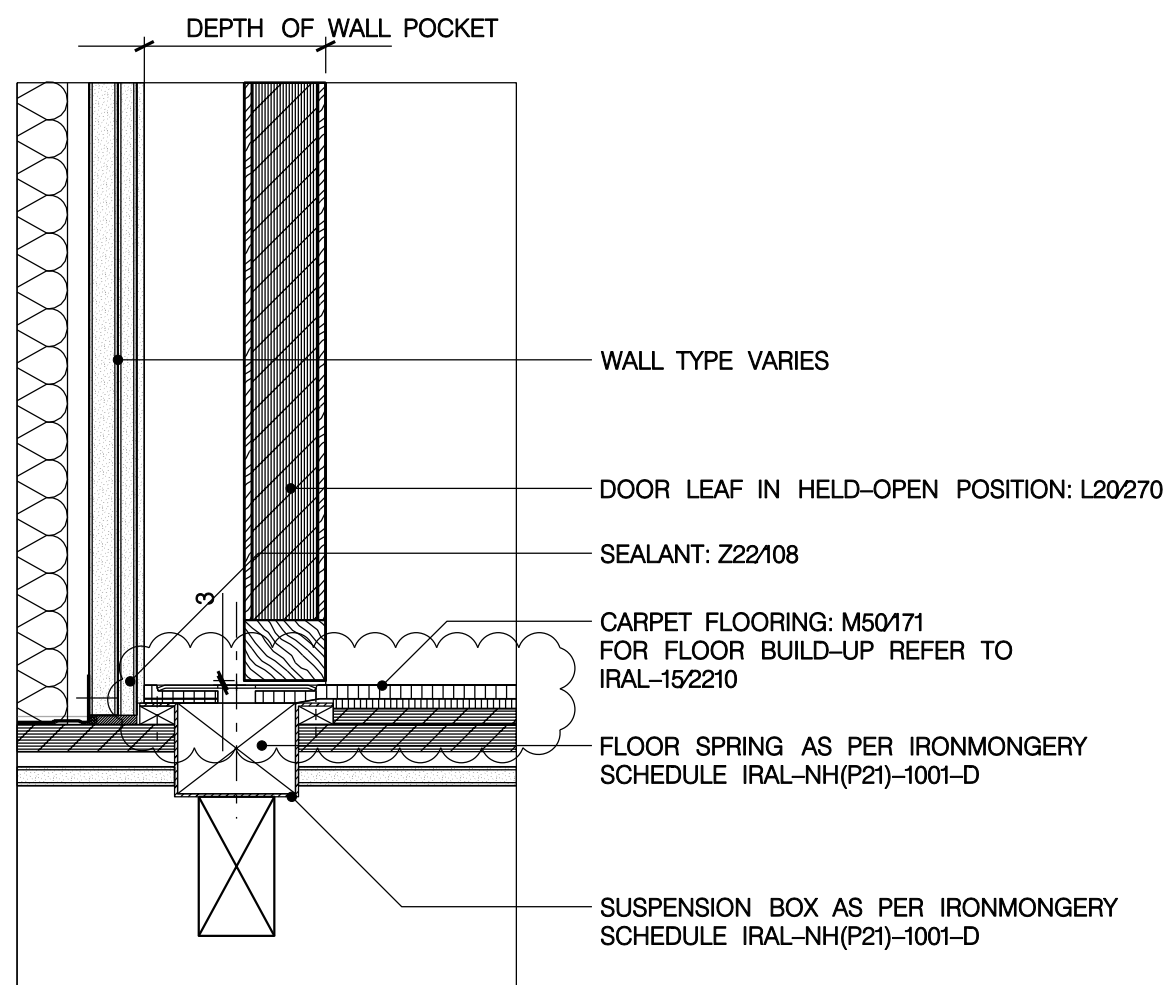
SECTION DETAIL FLOOR BOX DETAIL OF D-206-1, D-201-1, D-203-2, D-306-1, D-301-1, D-303-1
