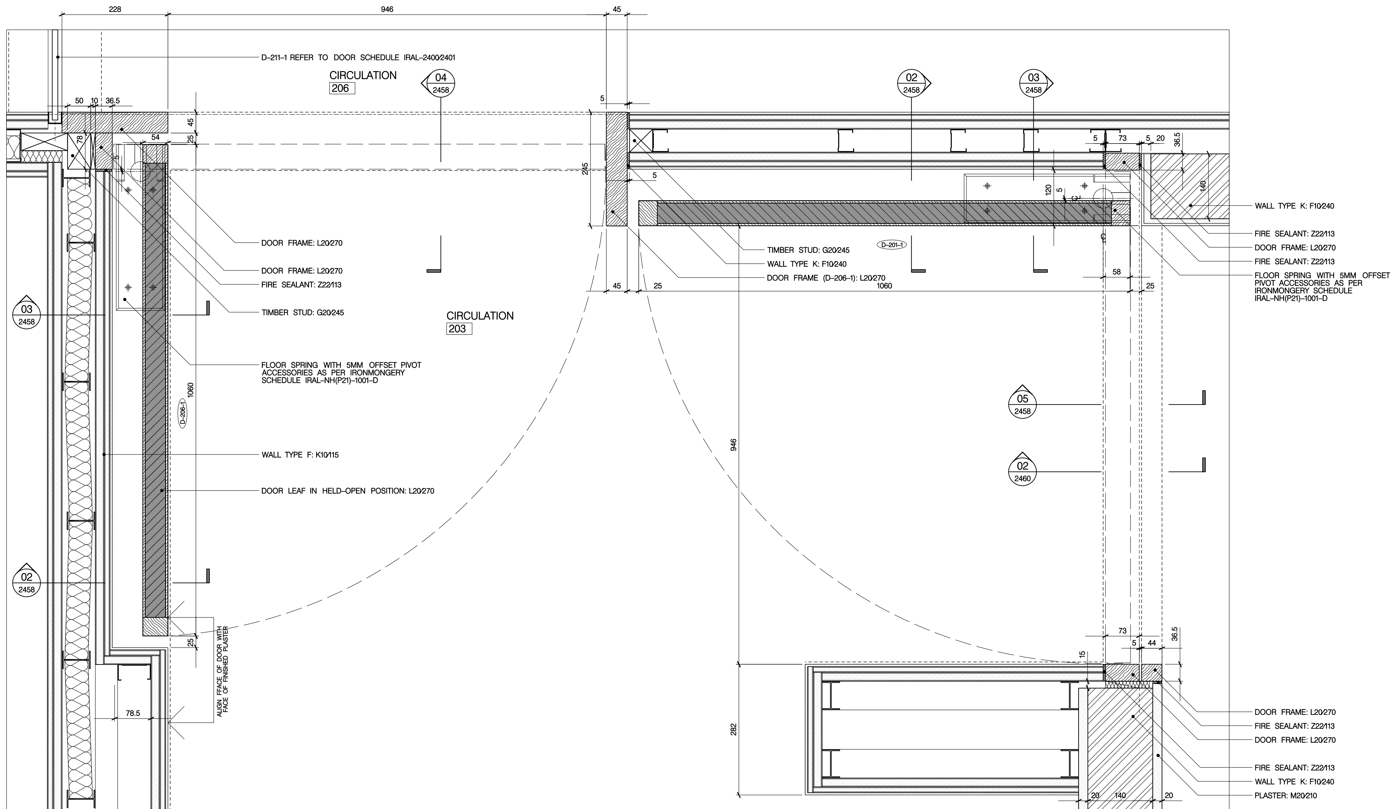
PLAN DETAIL PLAN DETAIL OF D-206-1 & D-201-1
