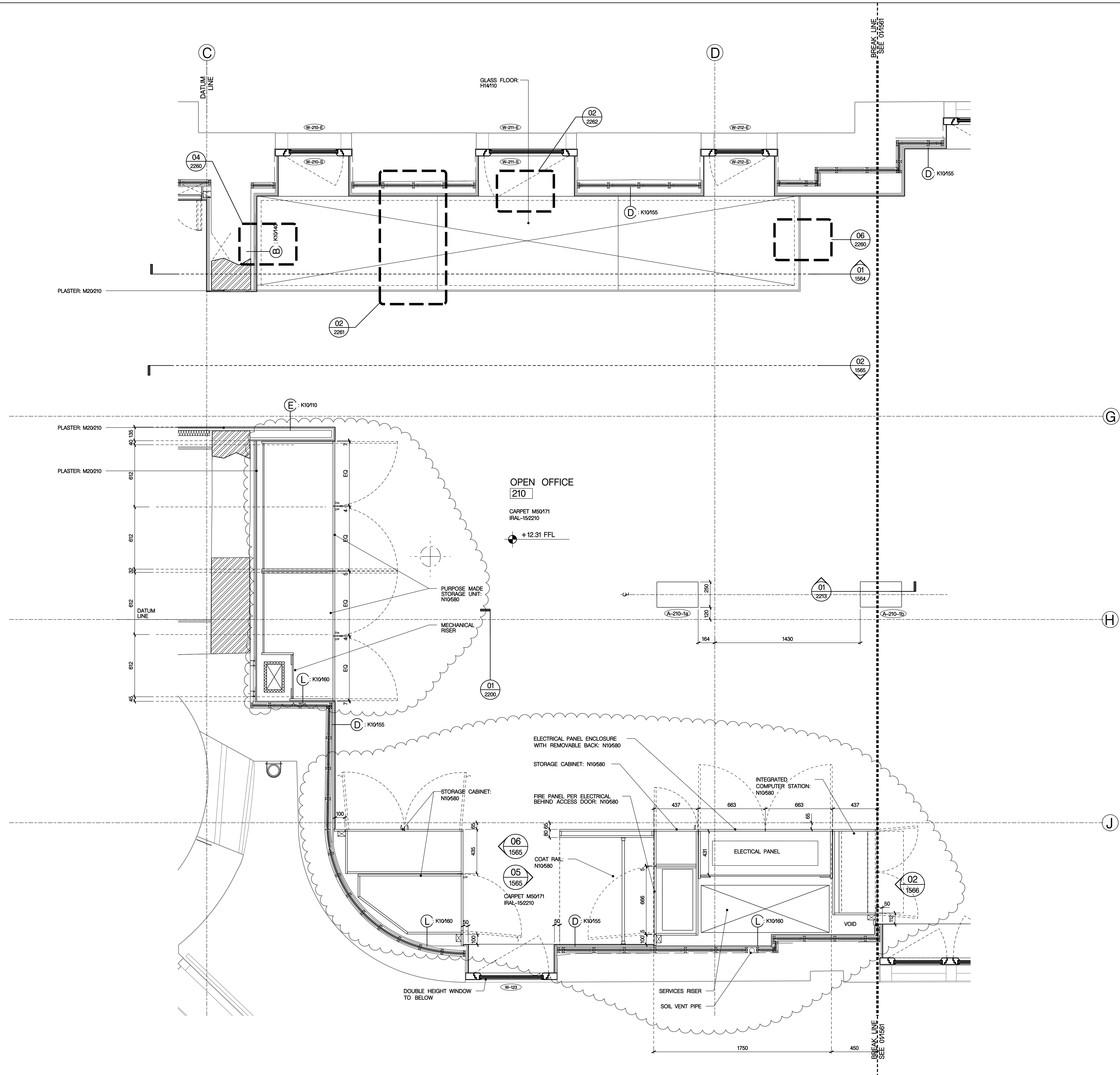
DETAILED FLOOR PLAN ROOM 210 - OPEN OFFICE
