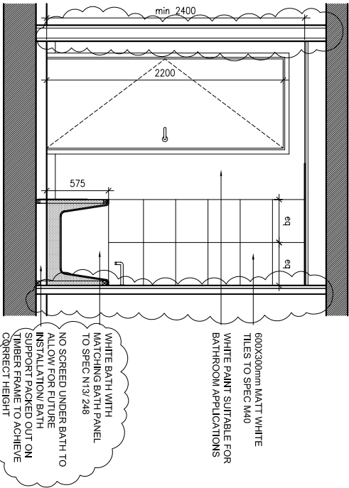
ELEVATION D
