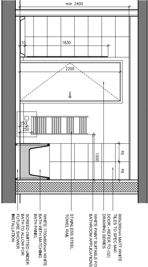
ELEVATION D
