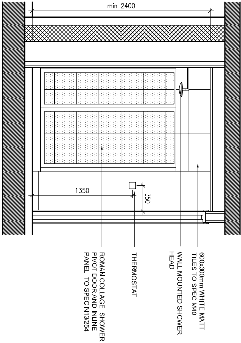
ELEVATION C
