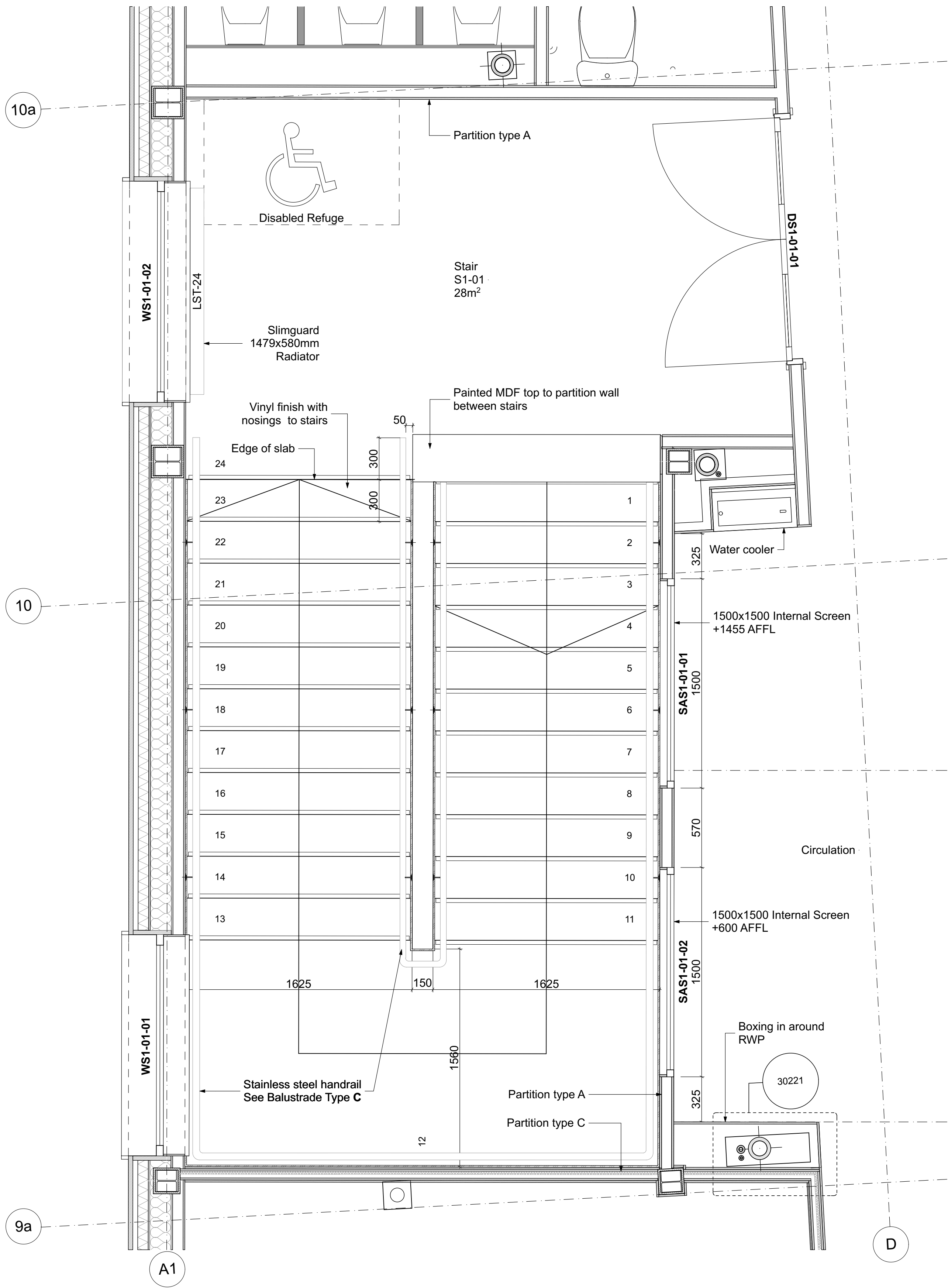
Stair ST01 First Floor
