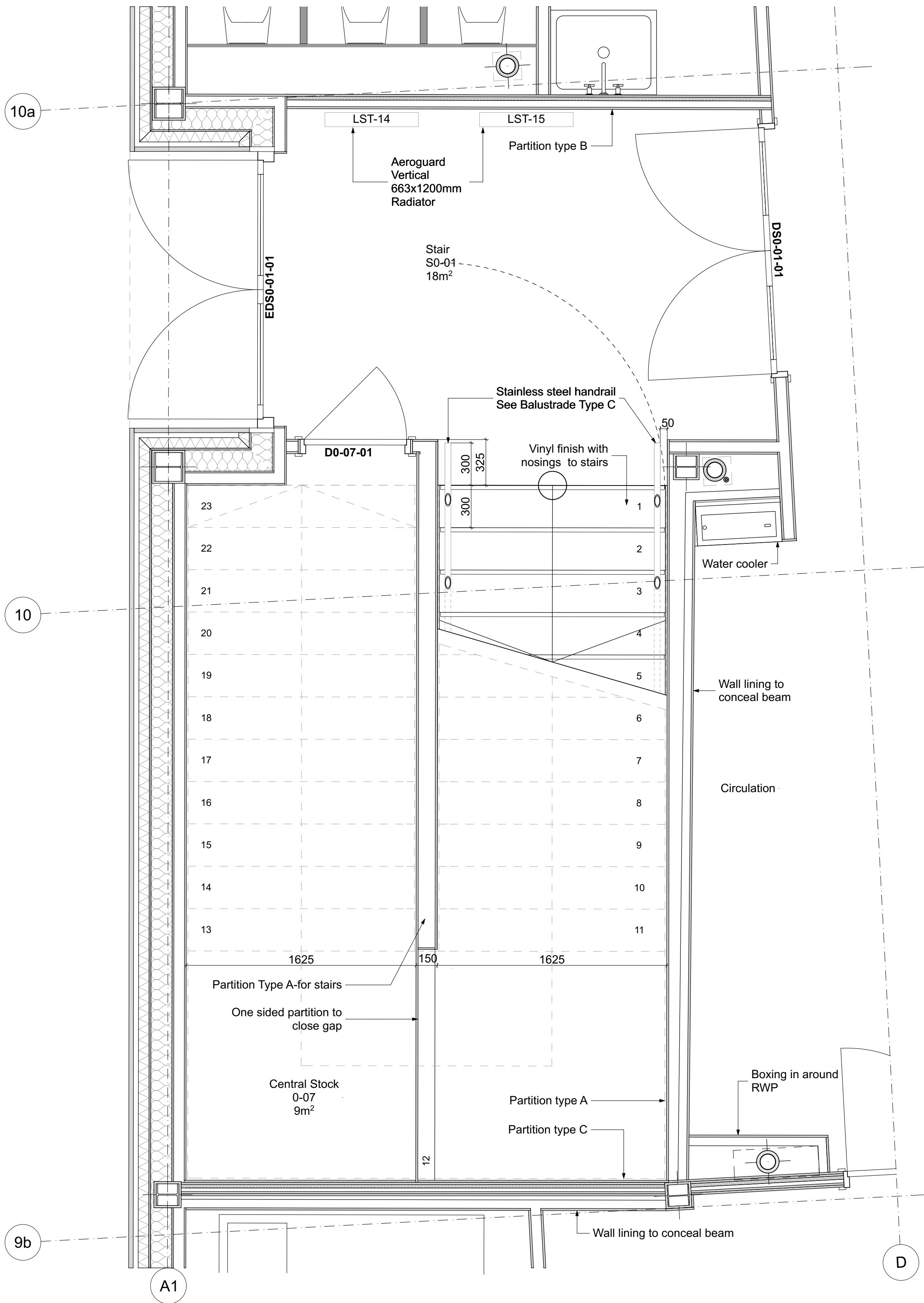
Stair ST01 Ground Floor
