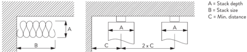
Wave stack depth - 2C roller cord (standard components)
