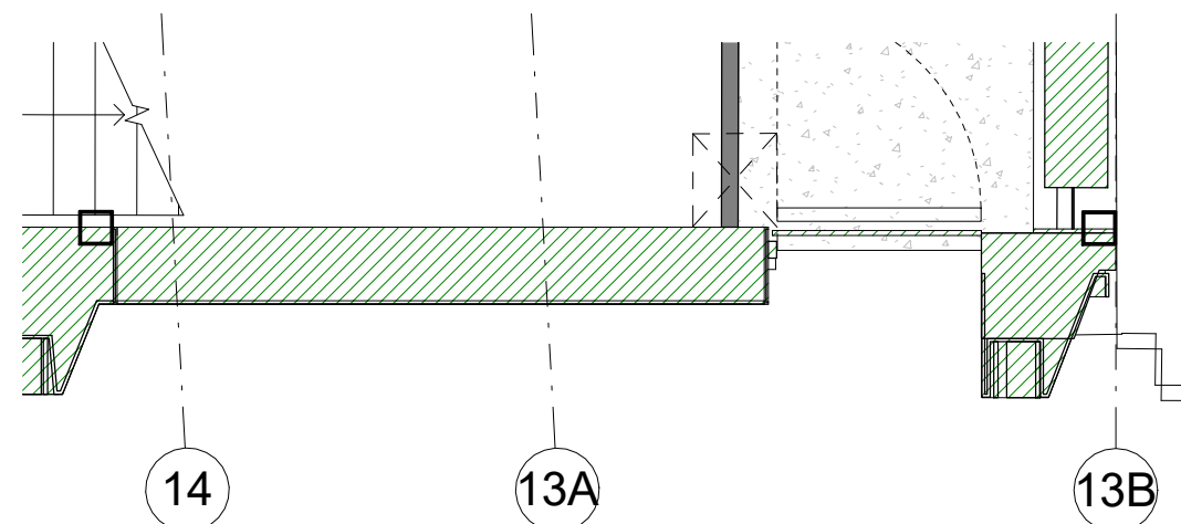
1 Facade - Ground Floor Plan
