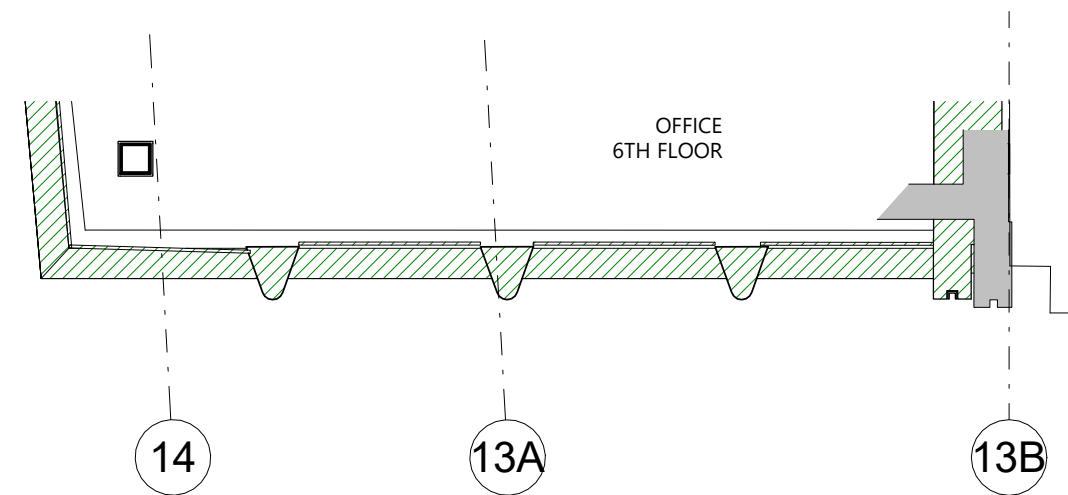
7 Facade - Sixth Floor Plan
