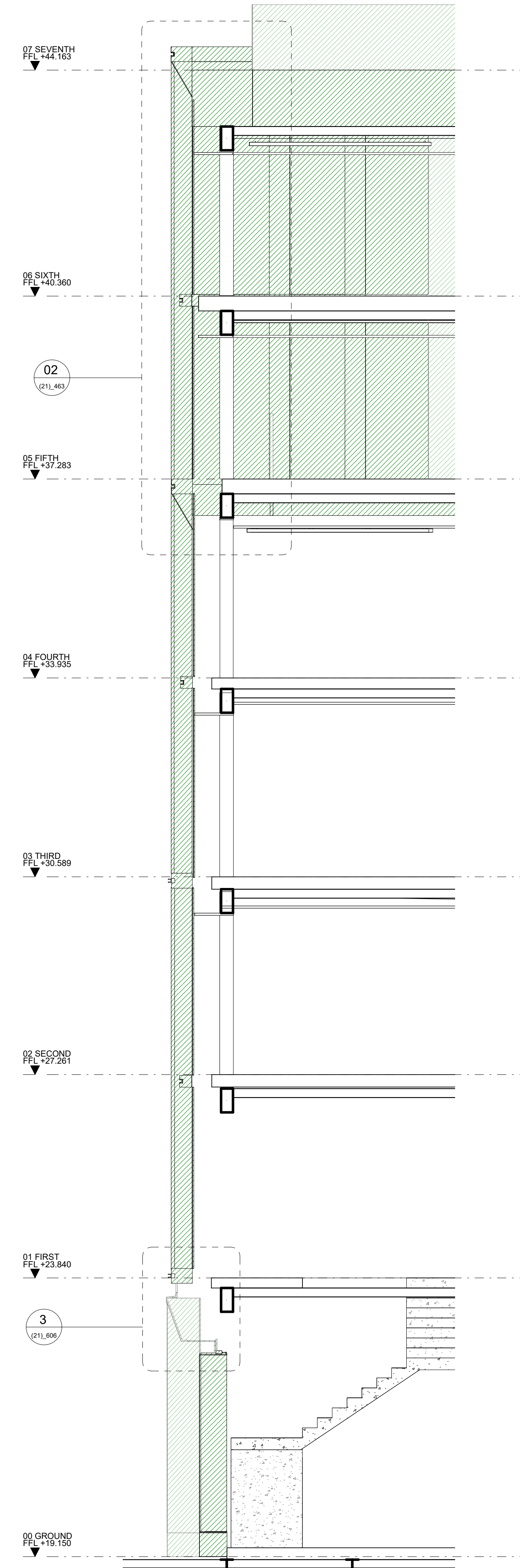
9 Pavilion Dover Street Section 1
