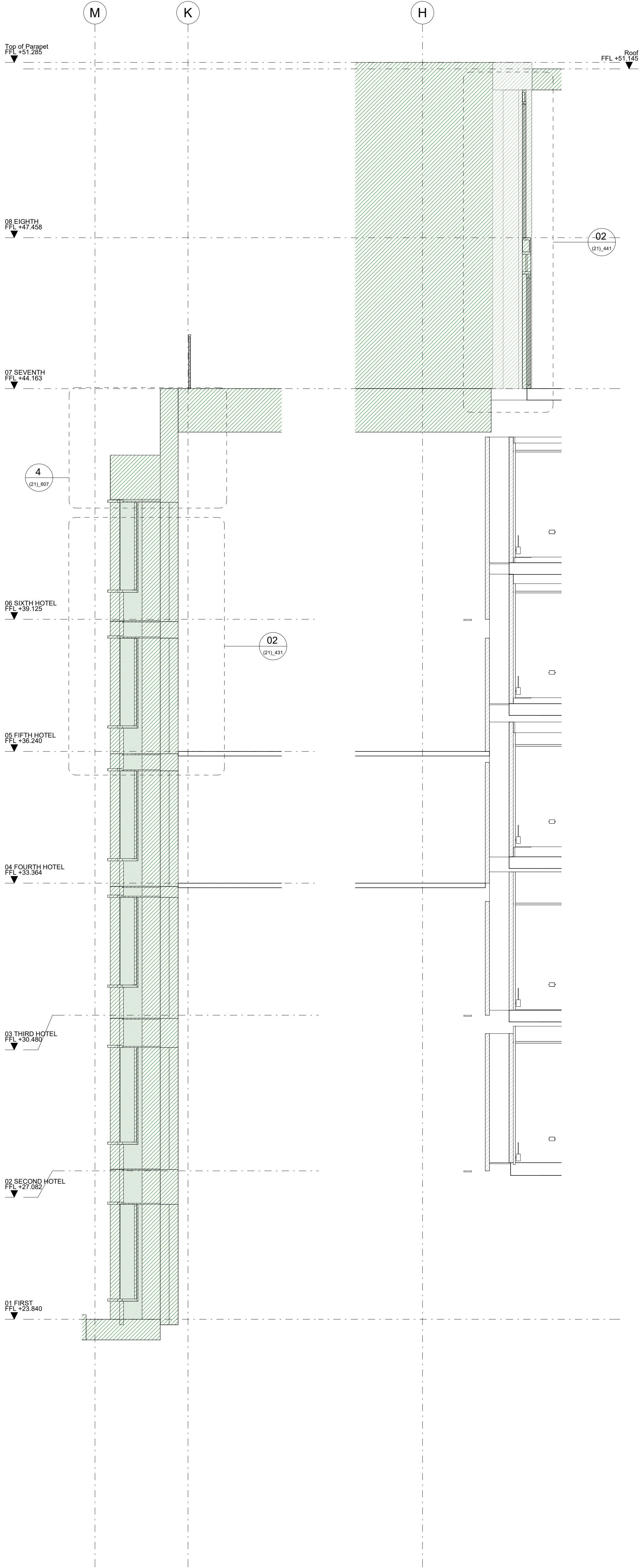
2 Dover Yard Bay Windows Section 1 : 50
