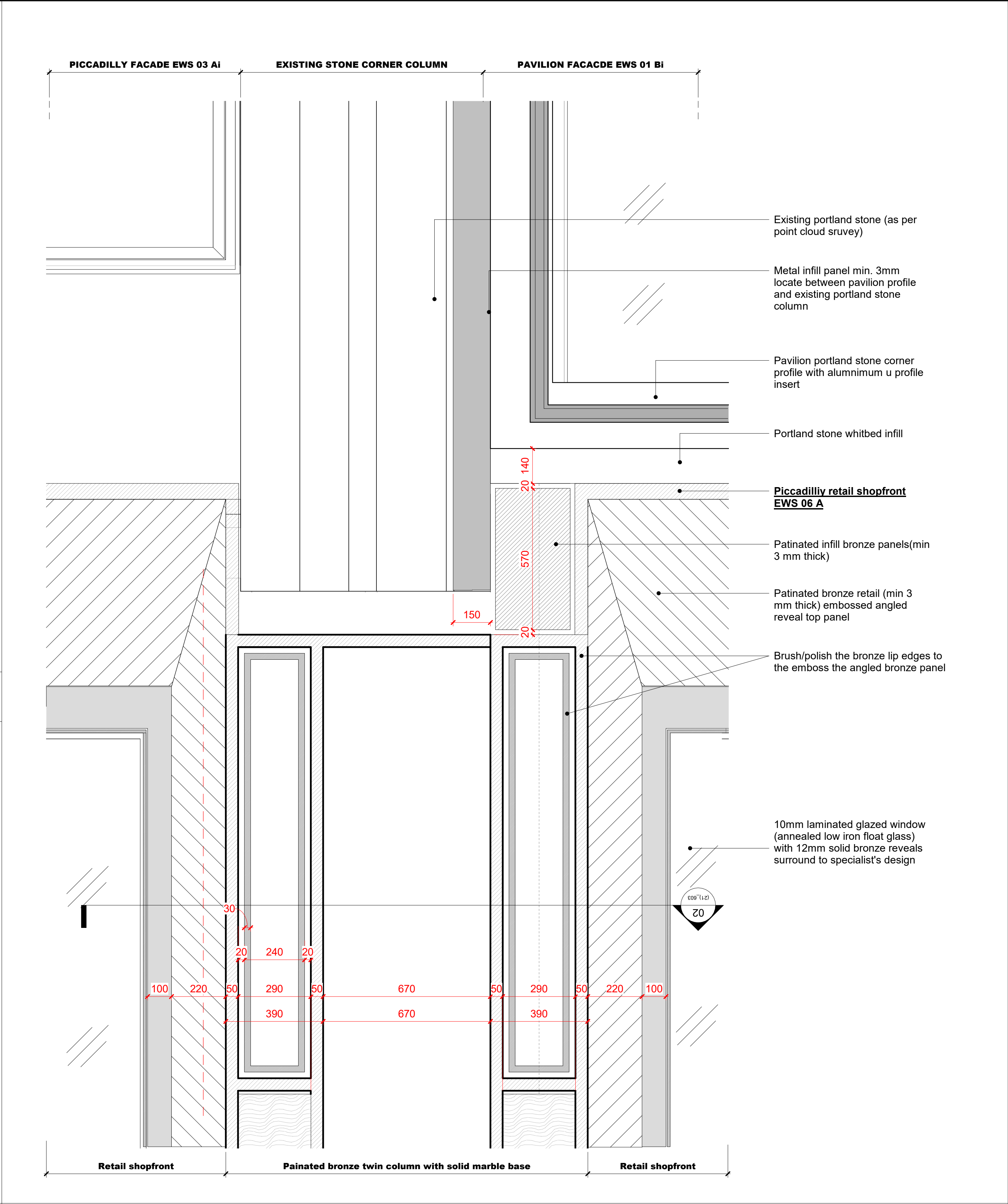
PICCADILLY RETAIL/PAVILION JUNCTION - ELEVATION 1 : 10 03
