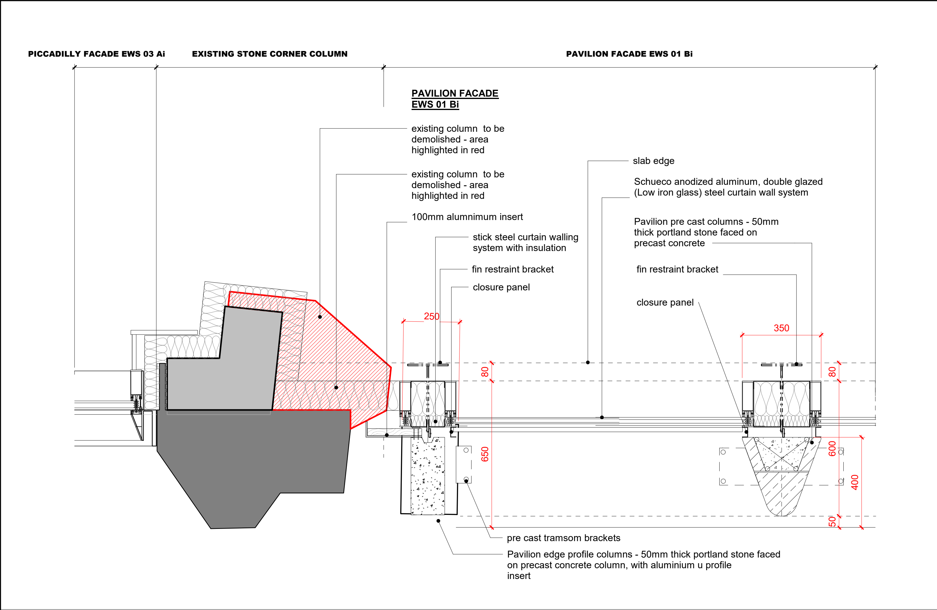
01 PICCADILLY RETAIL/PAVILION JUNCTION - PLAN 1 : 10
