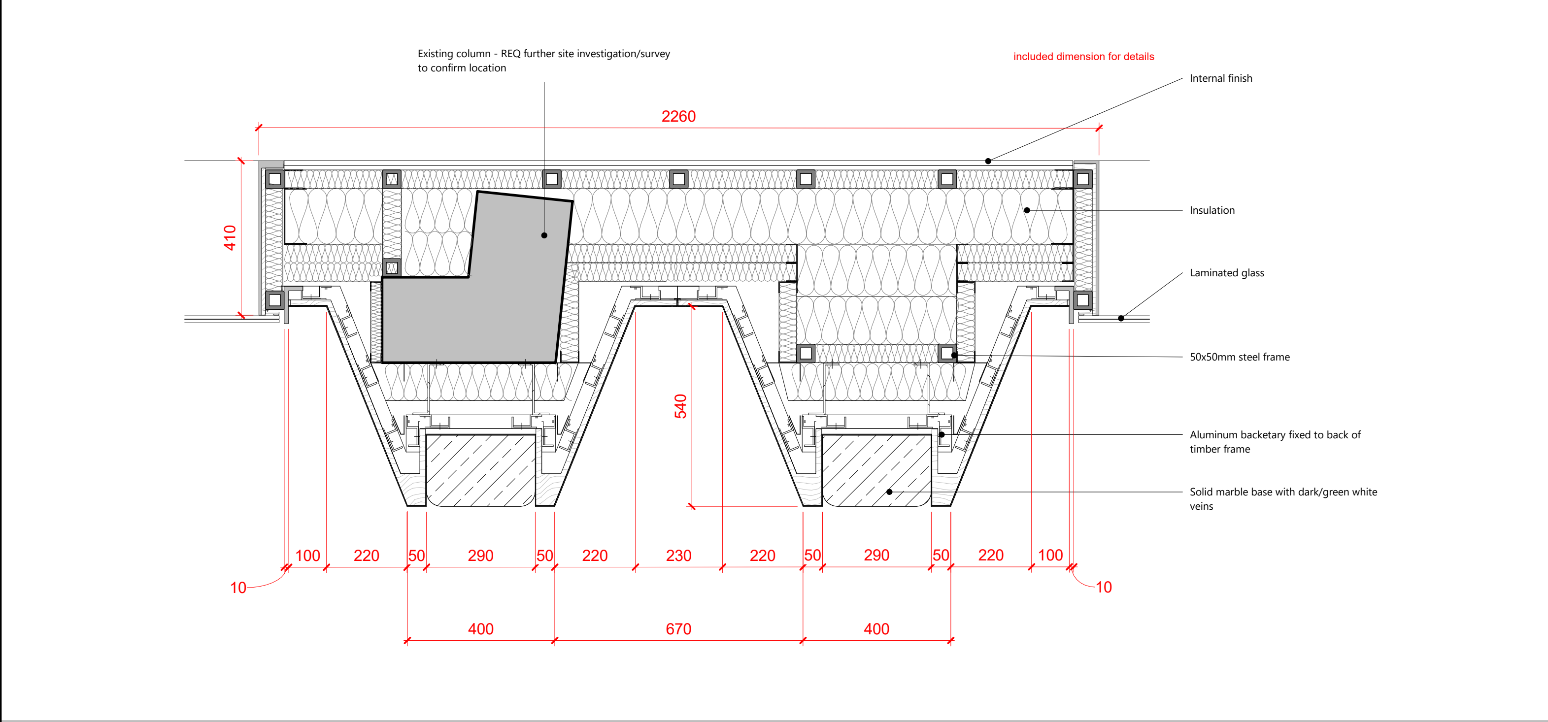
02 PICCADILLY RETAILTWIN COLUMN PLAN 1 : 10
