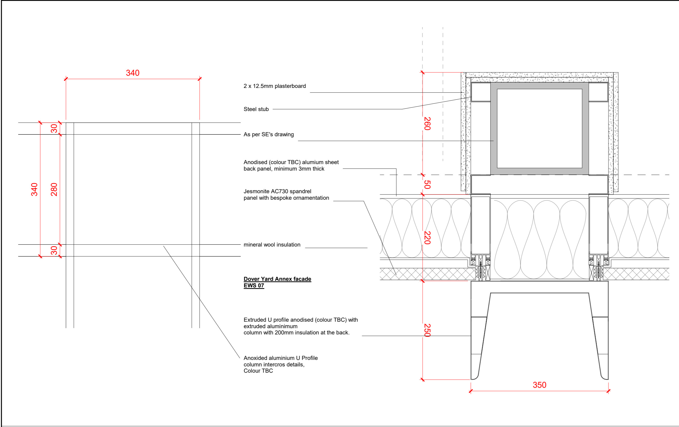
2 ANNEXE/DOVER YARD FACADE COLUMN DETAILS EWS 06 B & EWS 07
