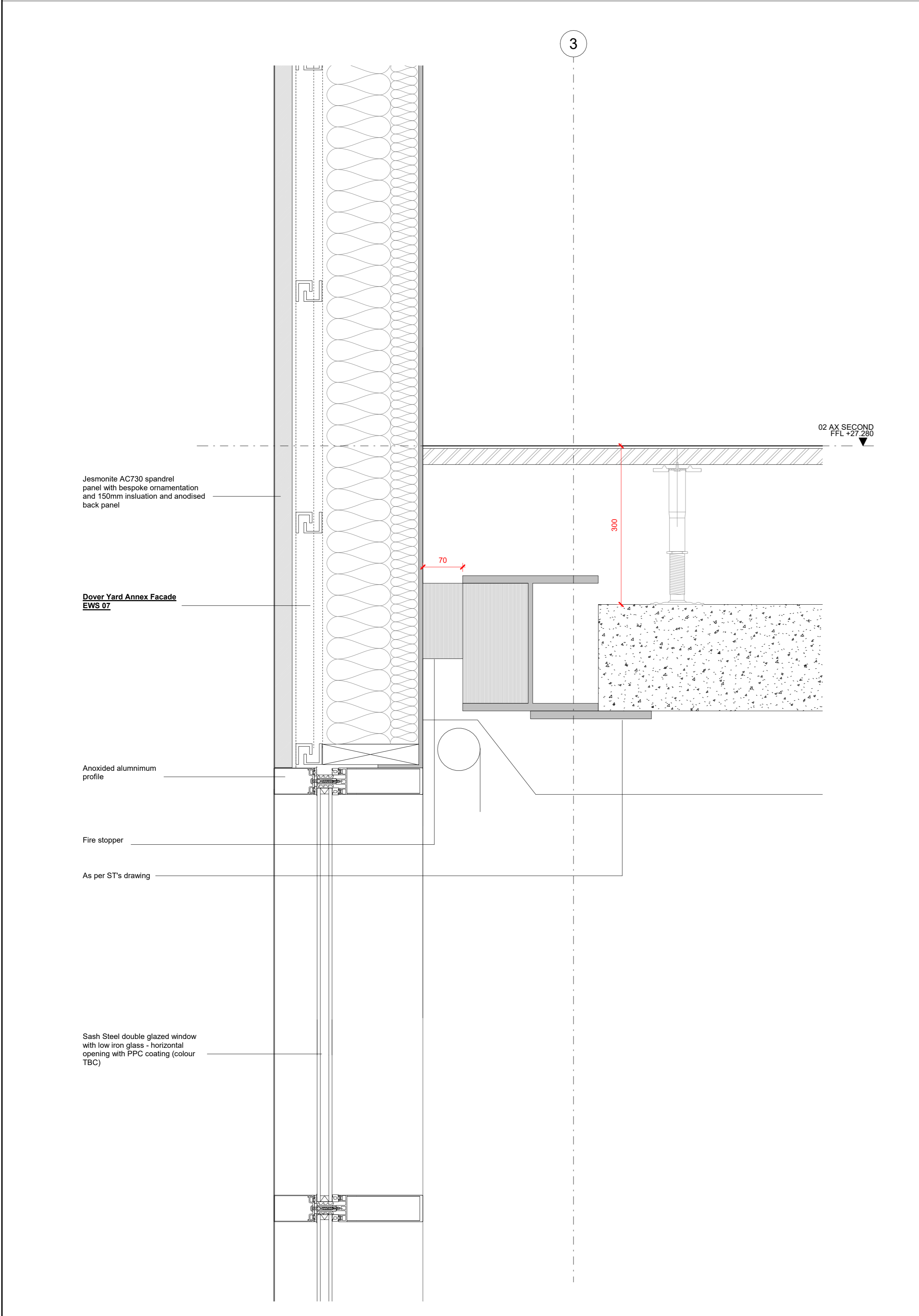
3 DOVER YARD ANNEX DETAILS- SECTION 1 : 5
