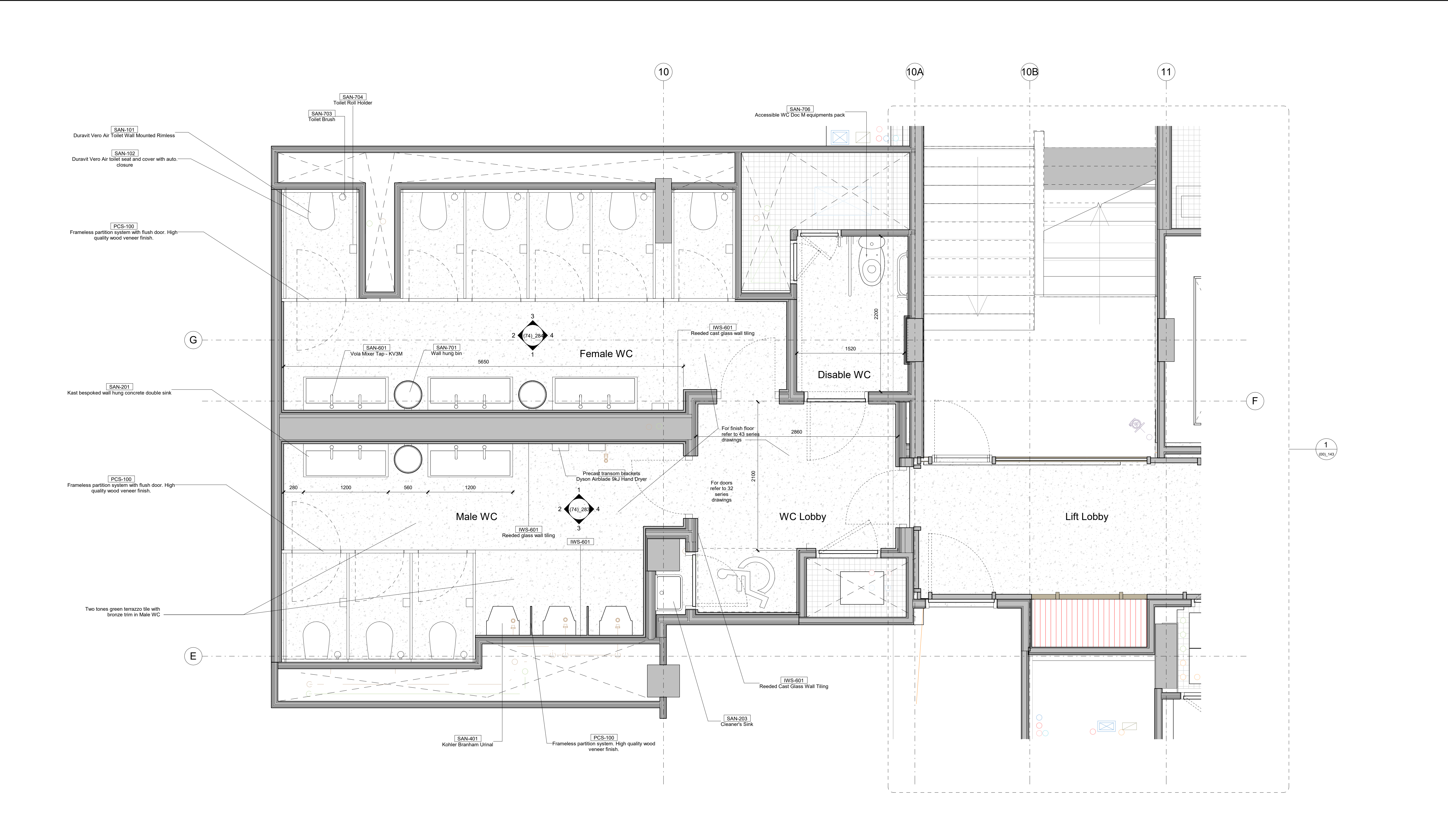
1 DETAIL CORE C WC PLAN 1 : 25
