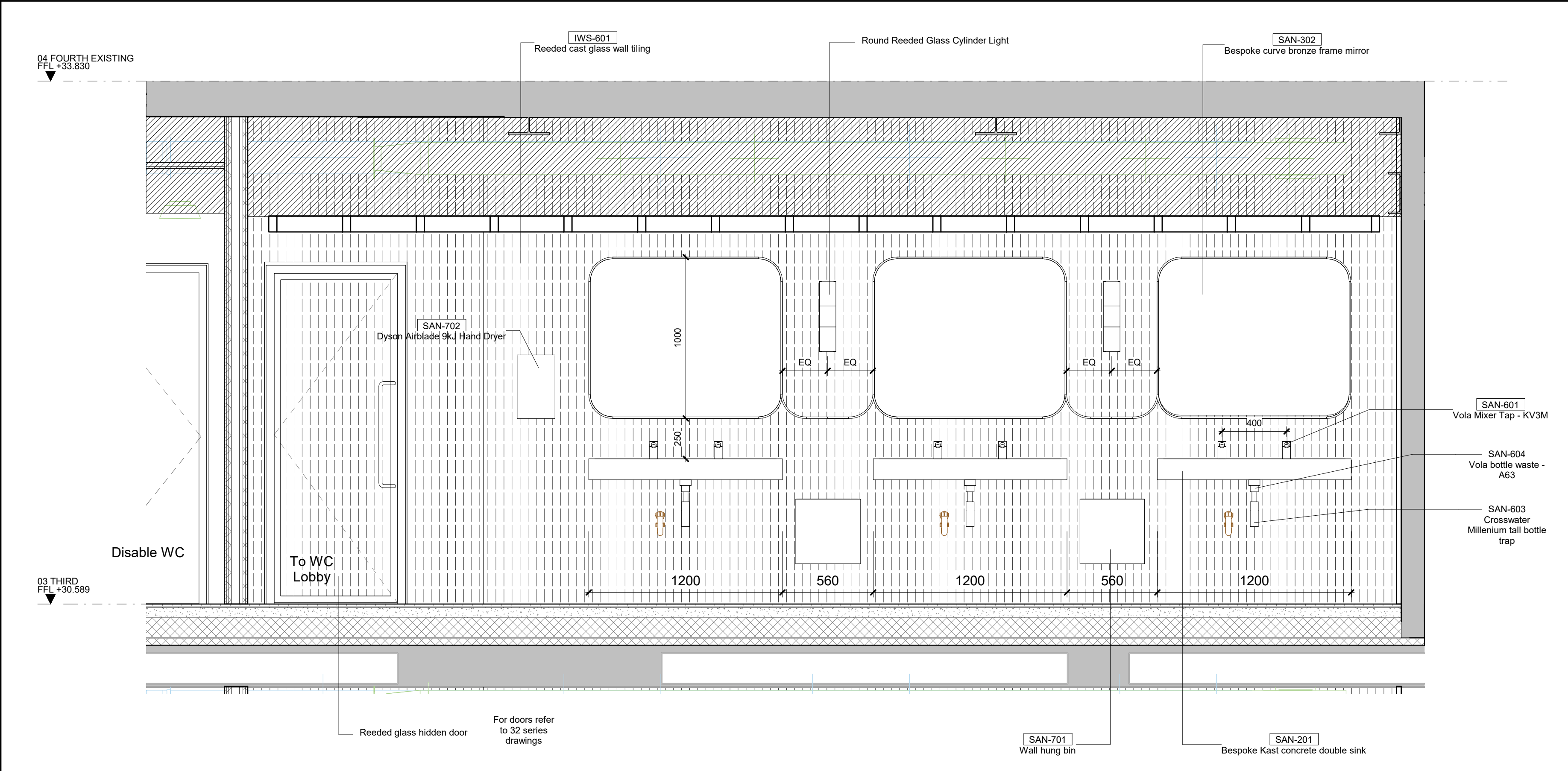
1 CORE C FEMALE WC ELEVATION 01 1 : 20
