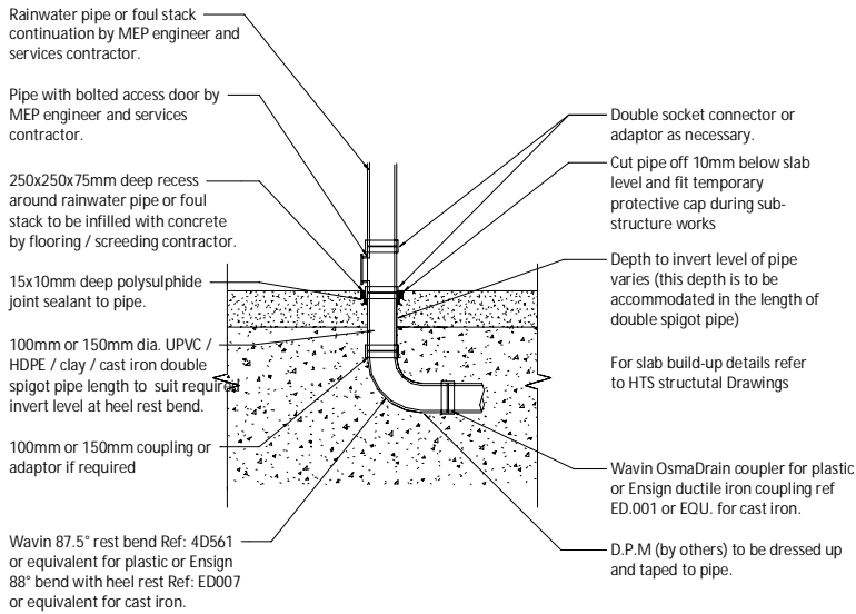
Typical Slab Penetration detail
