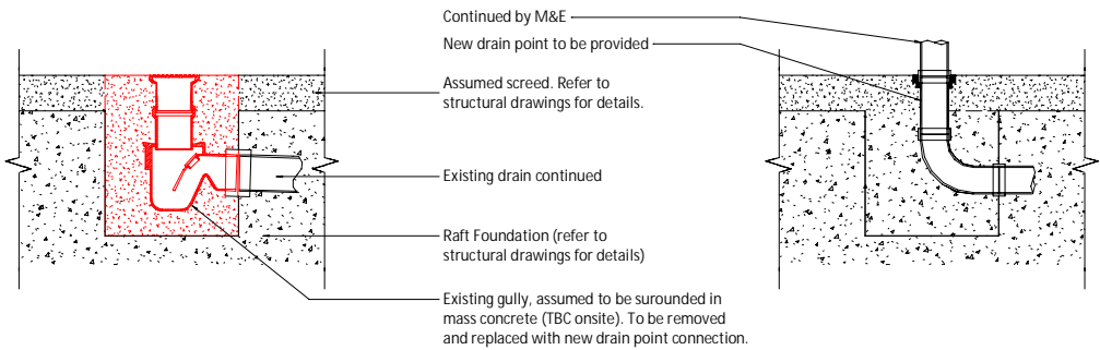
Typical Detail Showing a Floor Gully Replaced with a Drain Point
