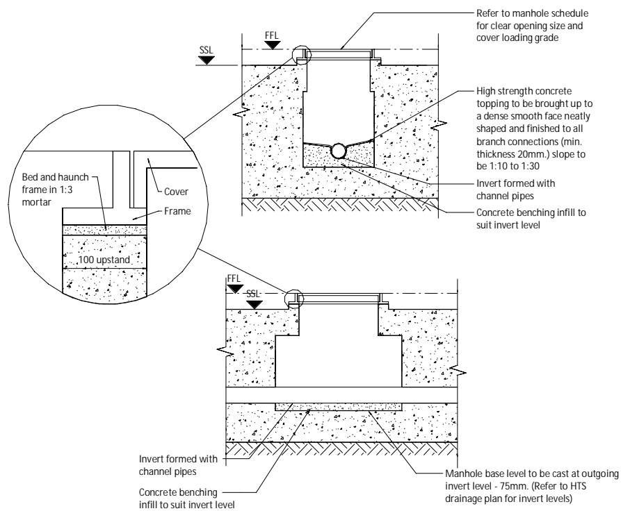
Typical In situ Manhole Detail
