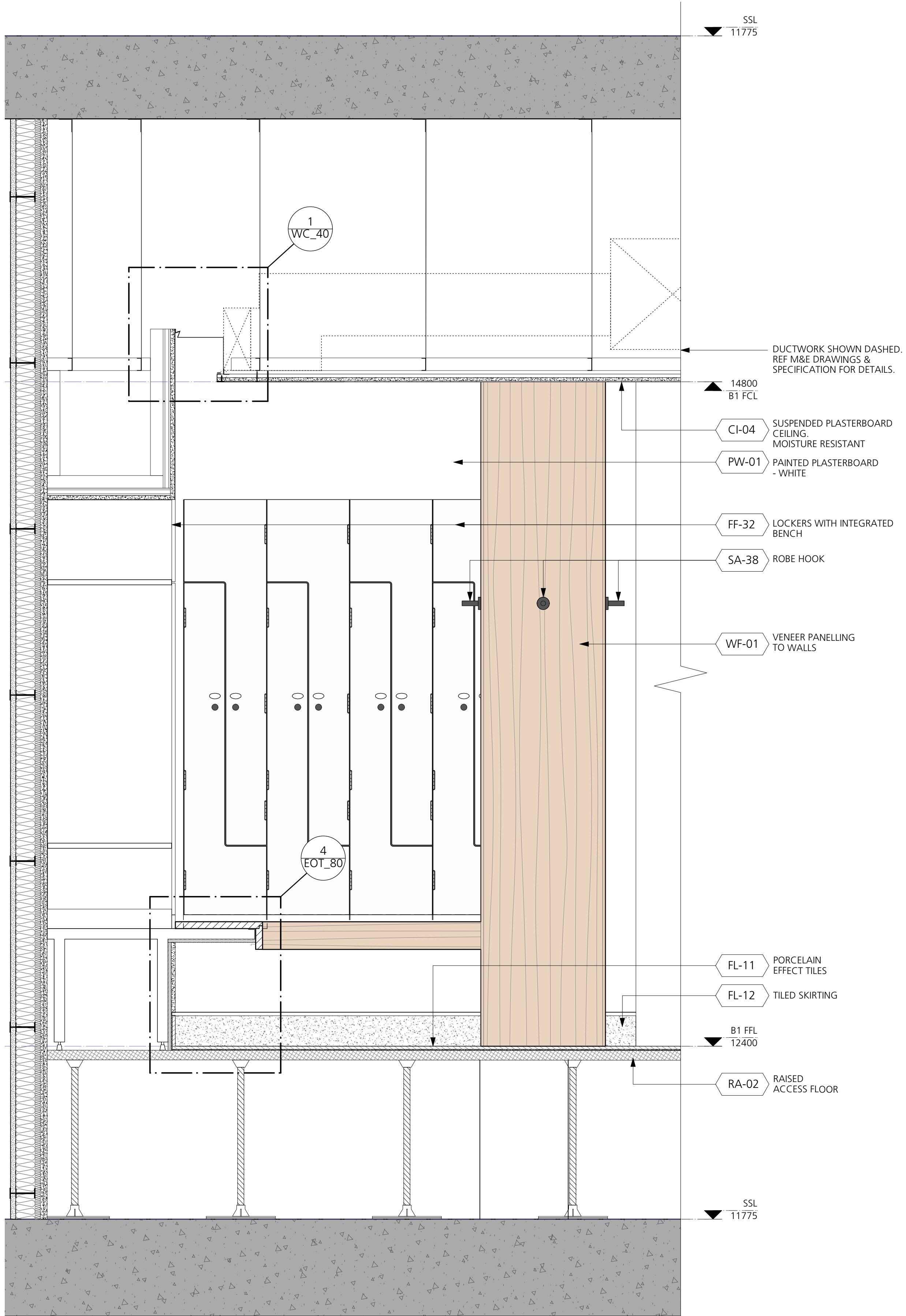
1 Typical Locker Detail Section Scale: 1:10
