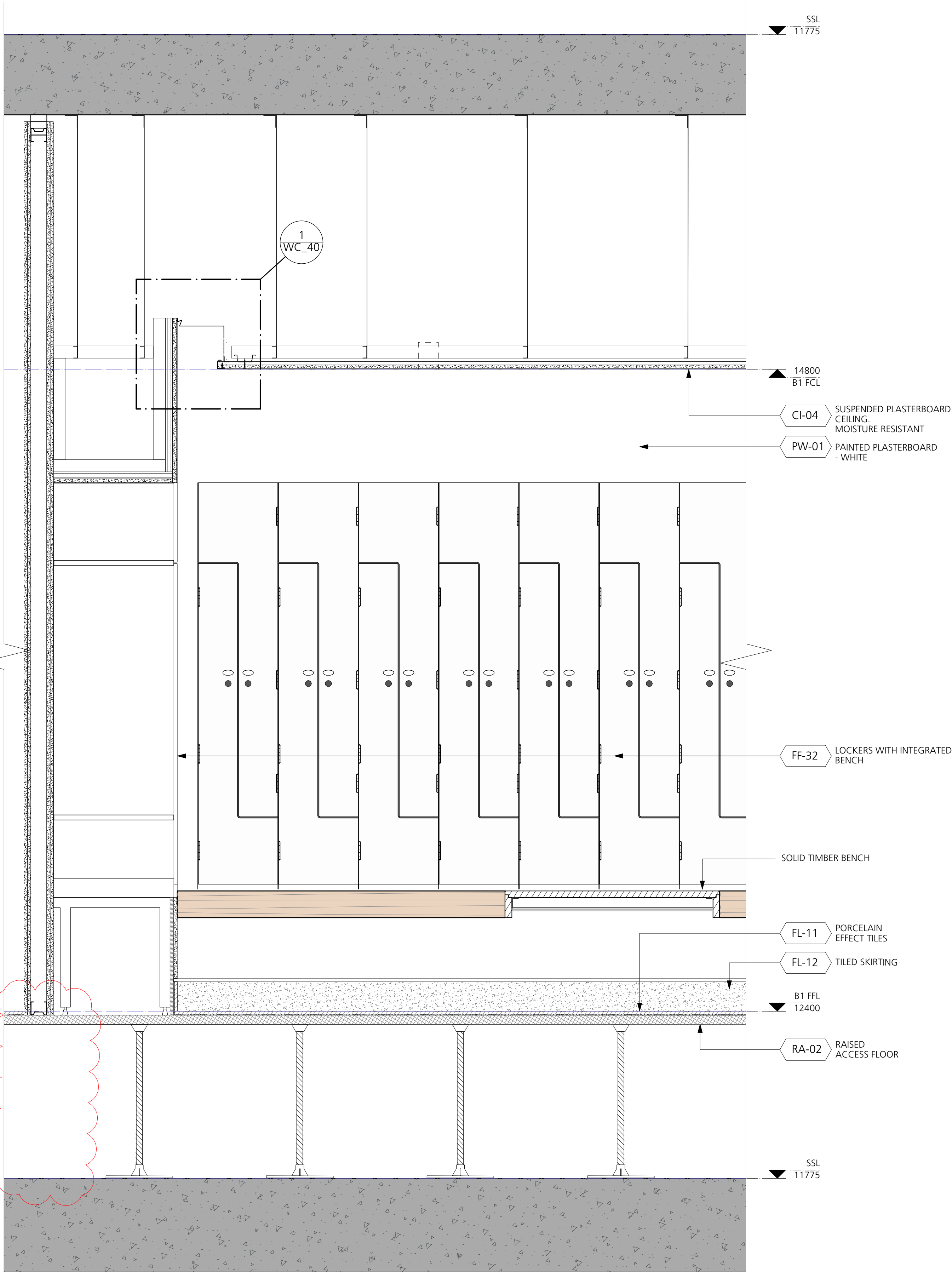
2 Typical Locker Detail Section Scale: 1:10
