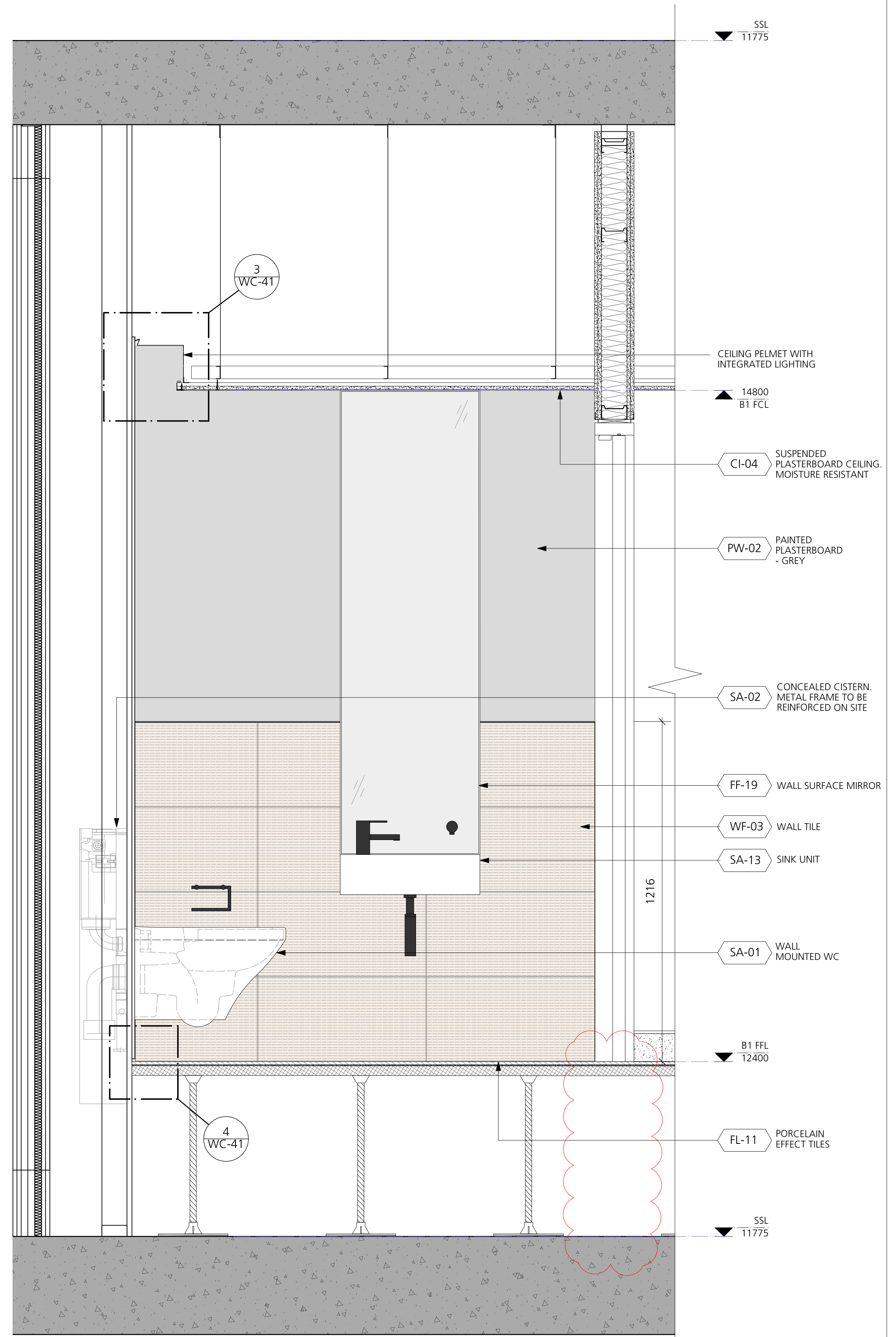
3 Typical WC Cubicle Elevation Scale: 1:10
