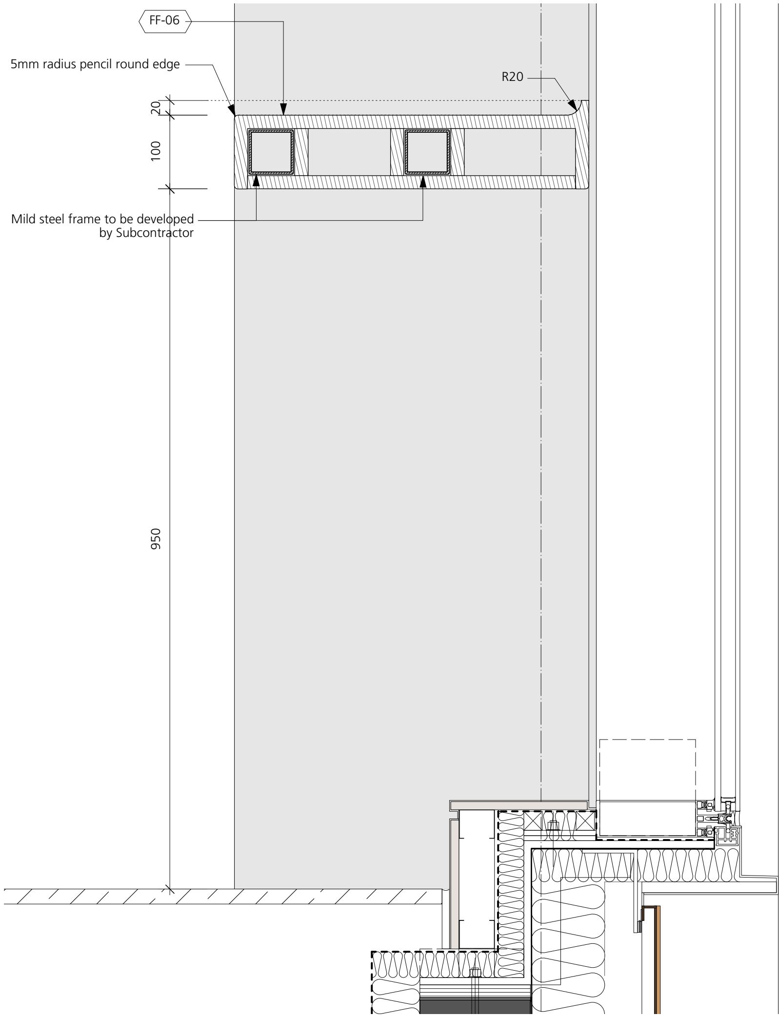
1 Window Bench Section Scale 1:5 @ A1
