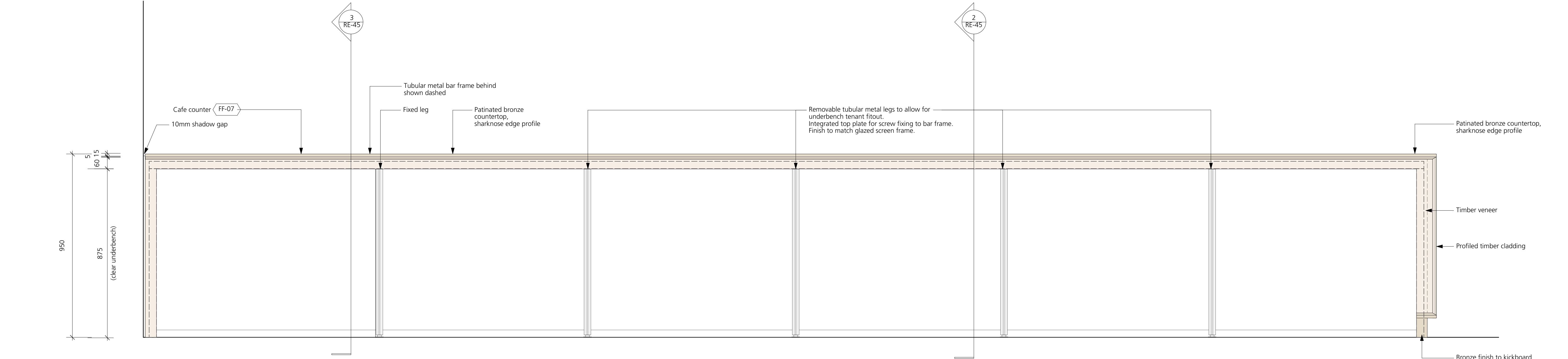
2 Cafe Counter Elevation Scale 1:10 @ A1
