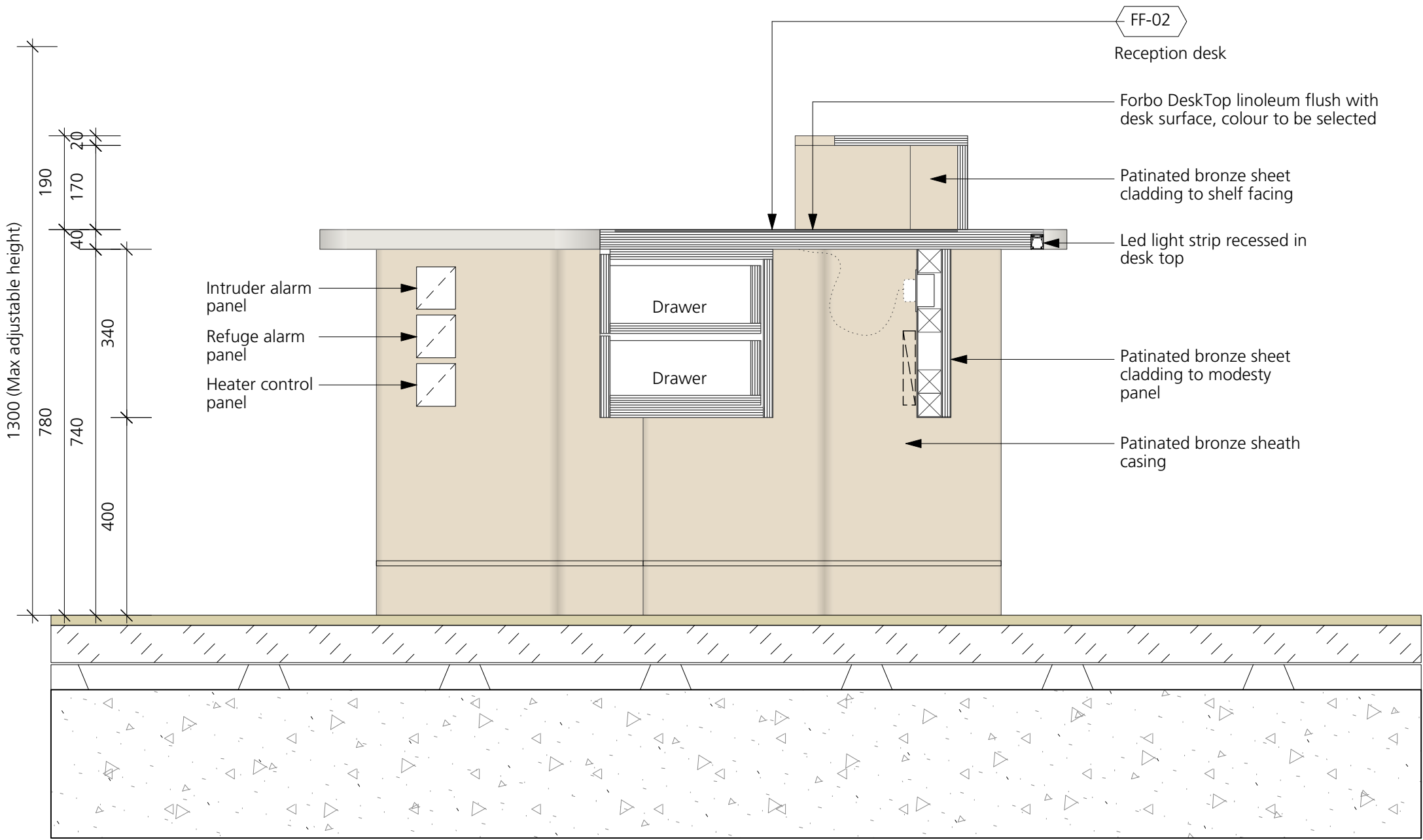
1 Reception Desk Section Scale 1:10 @ A1
