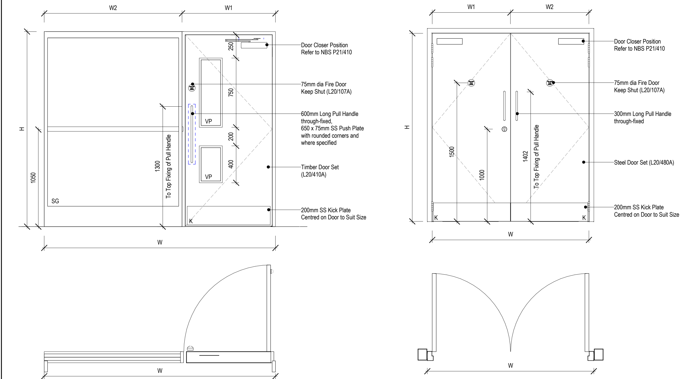
05 DOOR TYPE 205 - Single Door Set (w/ fixed Glazed Panel Core 1) SCALE 1:20
