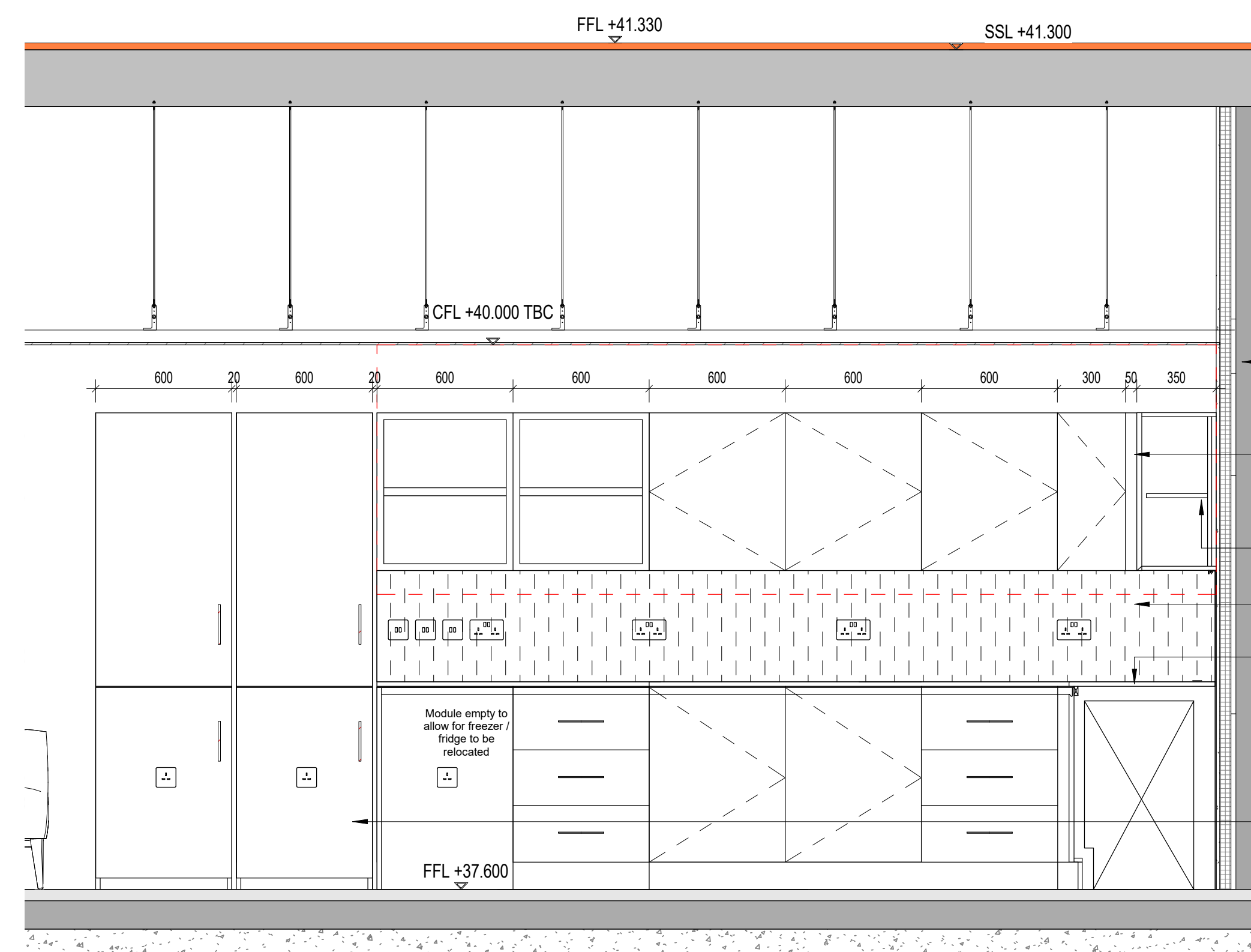
4 STAFF KITCHEN ELEVATION WEST Copy 1 EX(73)AL01 Scale: 1:20
