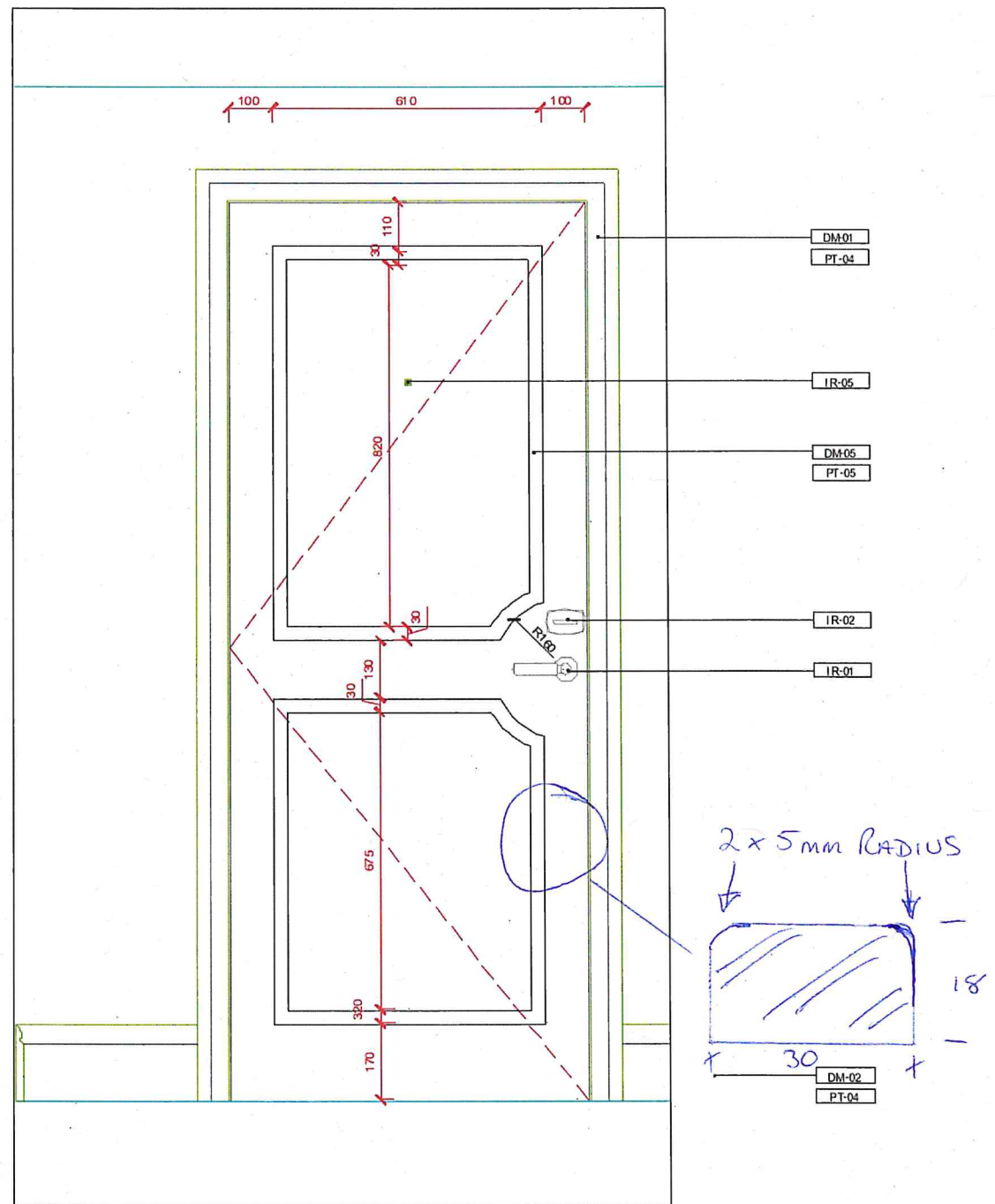
E2 | ELEVATION 02 - CORRIDOR SIDE SCALE 1:10
